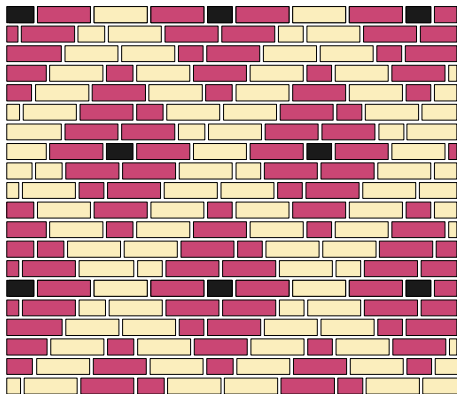
Triple Stretcher Garden Wall Bond with Units in Dovetail Fashion
