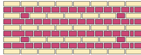
English Cross Bond
