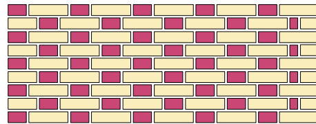
Flemish Bond
